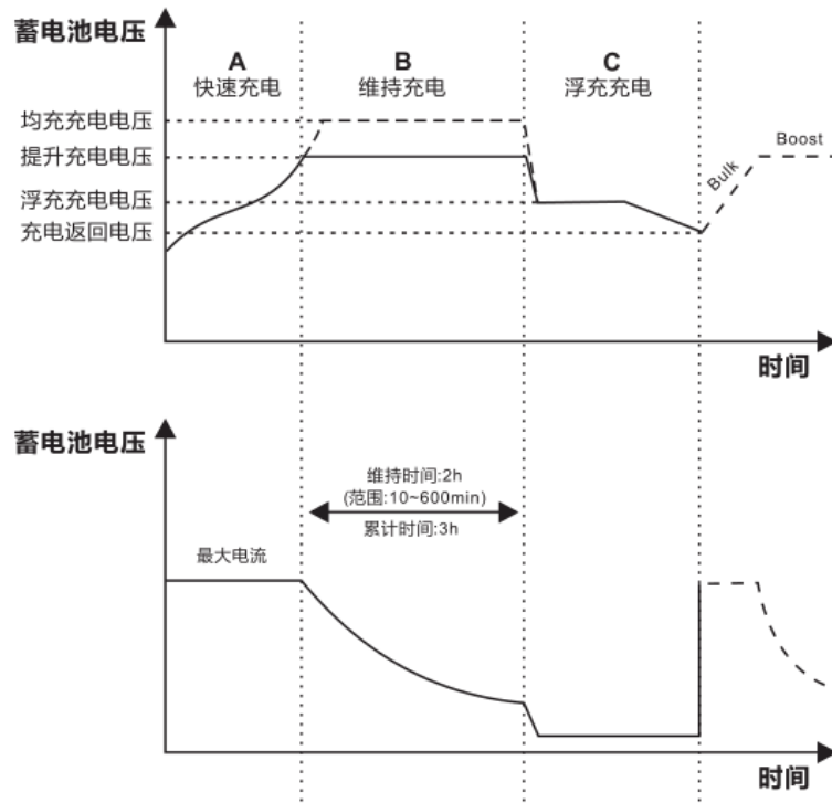
Fig. 1-5 Battery charging stages diagram
